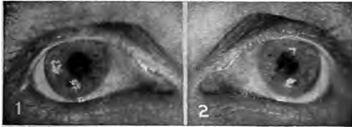
FIG. 32. REFLECTION OF THE ELECTRIC FILAMENT FROM THE IRIS
